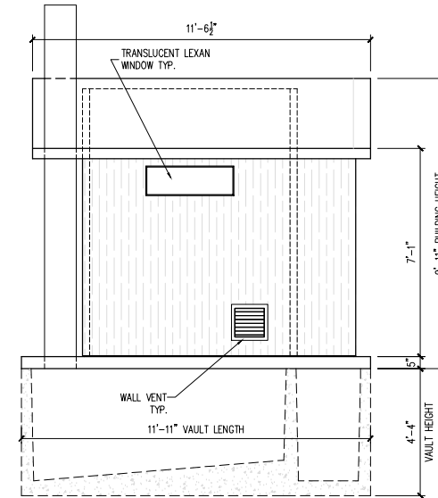
LEFT ELEVATION
