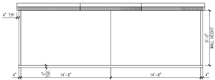
LEFT ELEVATION
