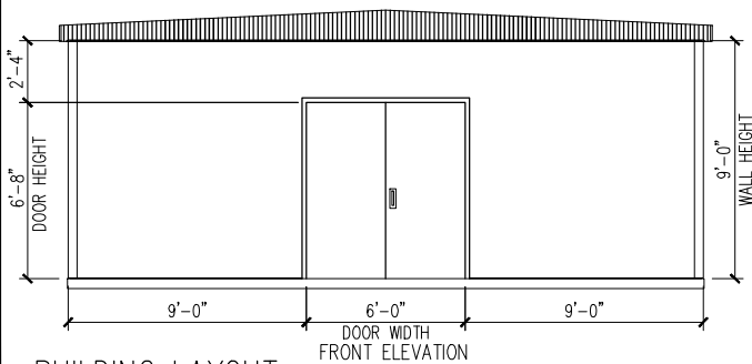
BUILDING LAYOUT
